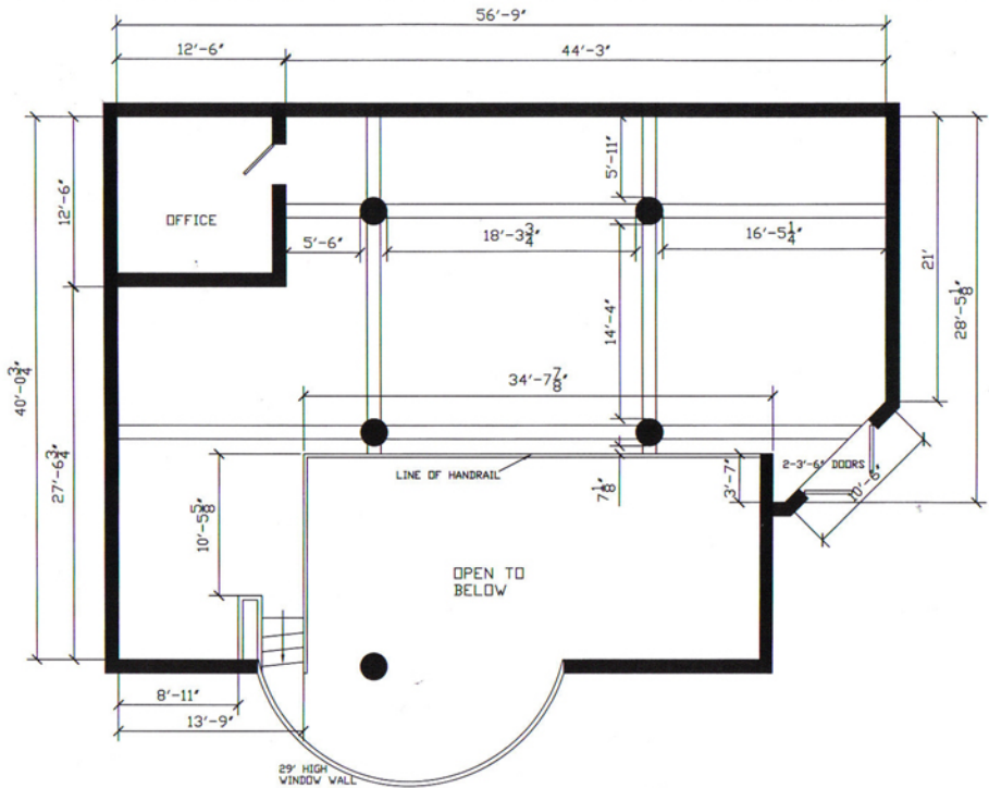
ELAINE L. JACOB GALLERY SECOND FLOOR PLAN WITH DIMENSIONS
